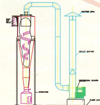
Cyclone Separator
